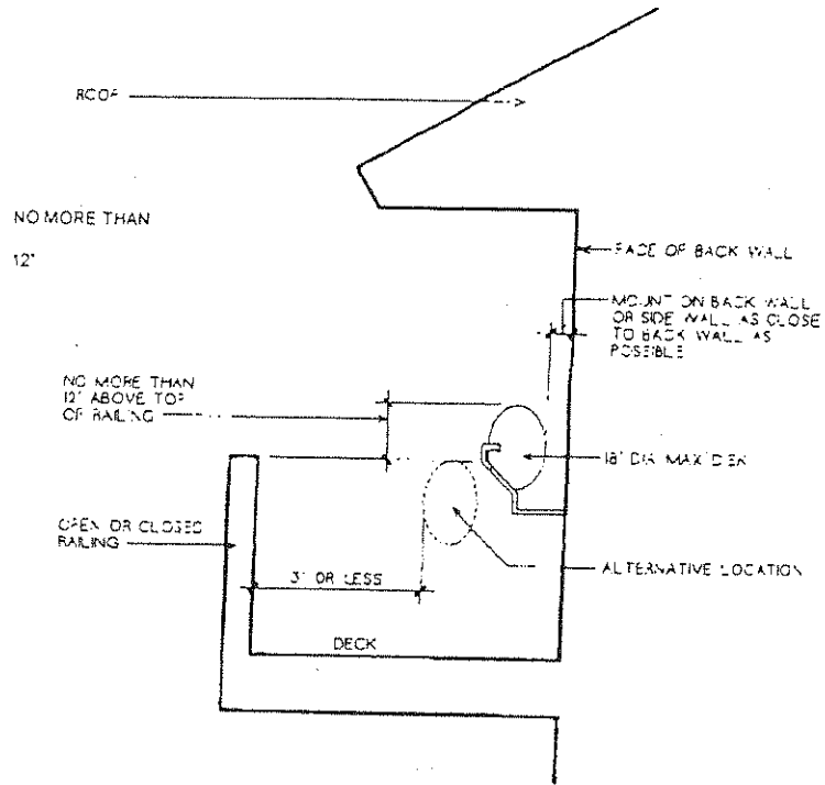
SECTION THRU TYPICAL DECK SCALE: 1/2" = 1'-0"
